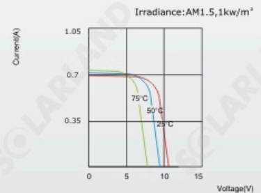
SLP005-06U I-V Curves
